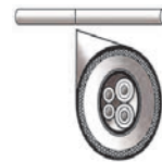
Guaranteed for Life™ headset cord cross-section
